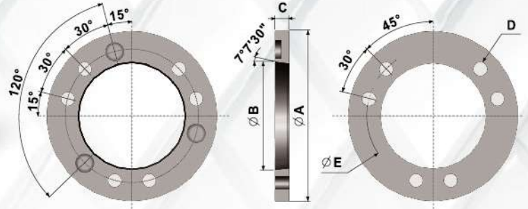
Fig1 適用於夾頭相對應標準大小主軸 The chuck is directly mounted onto the spindle nose.
